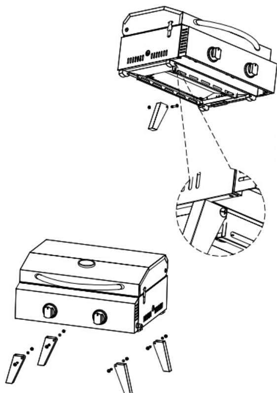
Fig.1 :Installing the foot stand legs as below showing.
