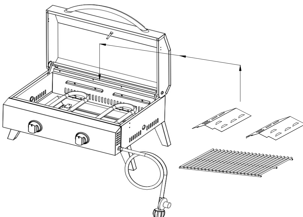
Fig3: Putting the flame tamer on the burner then put the grid on the firebox as below showing:
